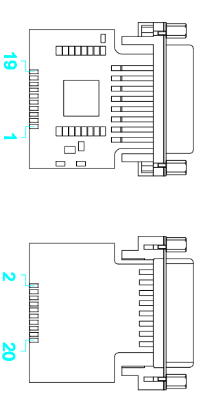
PCB: PTN3361
